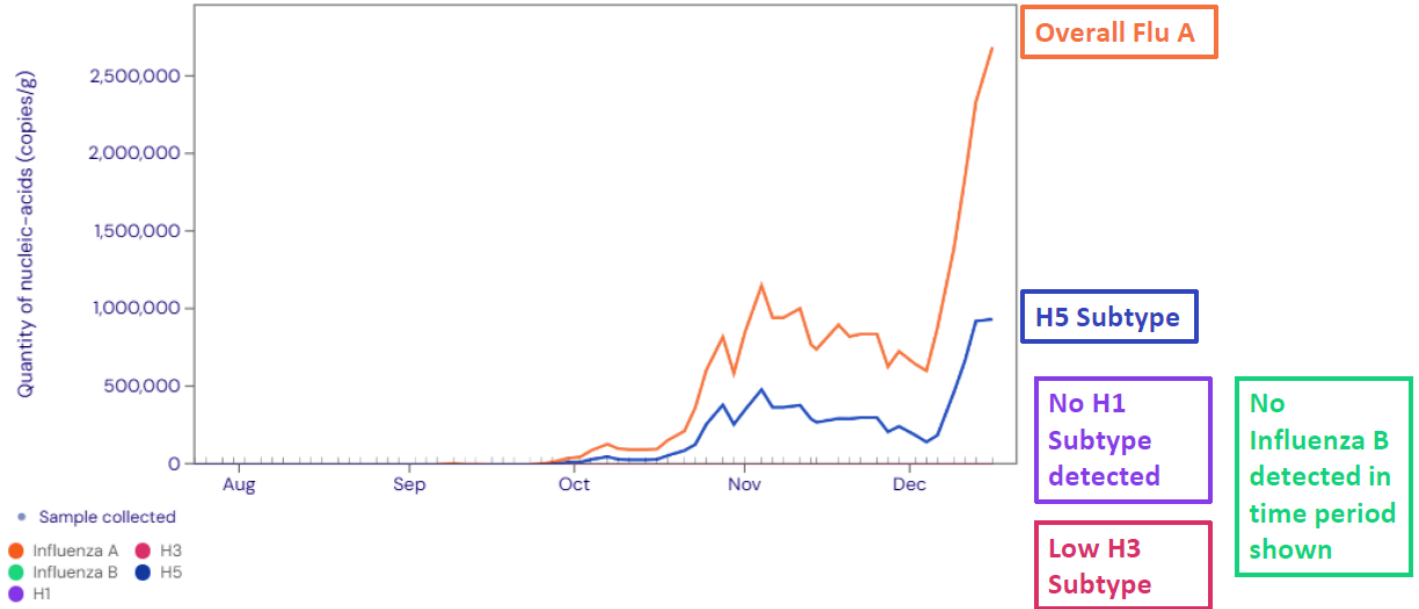
Influenza A with Subtypes H1, H3, and H5 (Turlock, CA)
